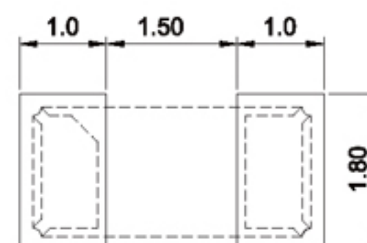
Top View Suggested Layout
